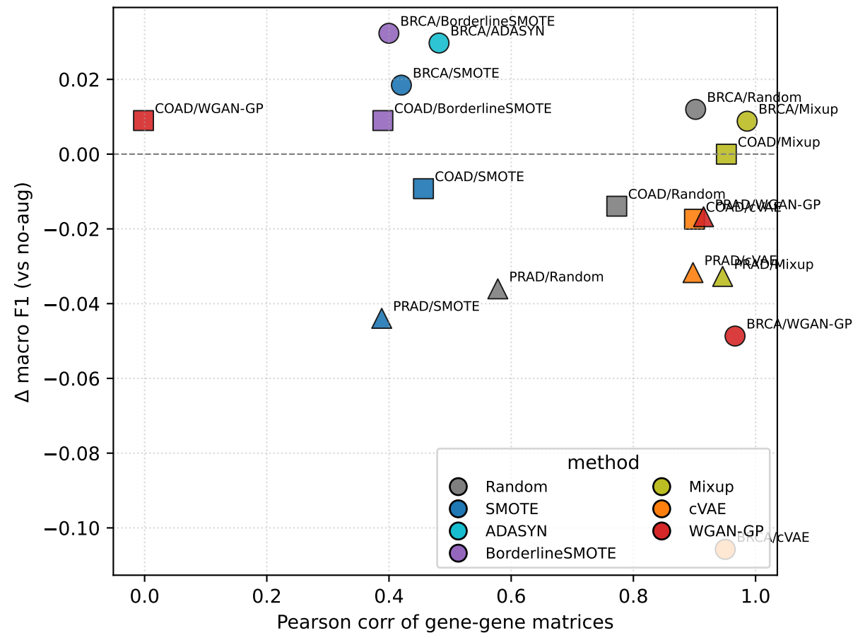
Correlation preservation vs downstream \Delta F1
