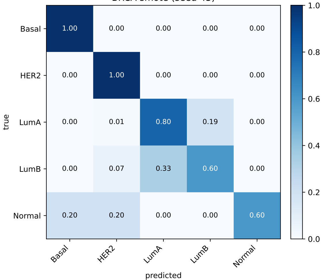
BRCA smote (seed 43)
