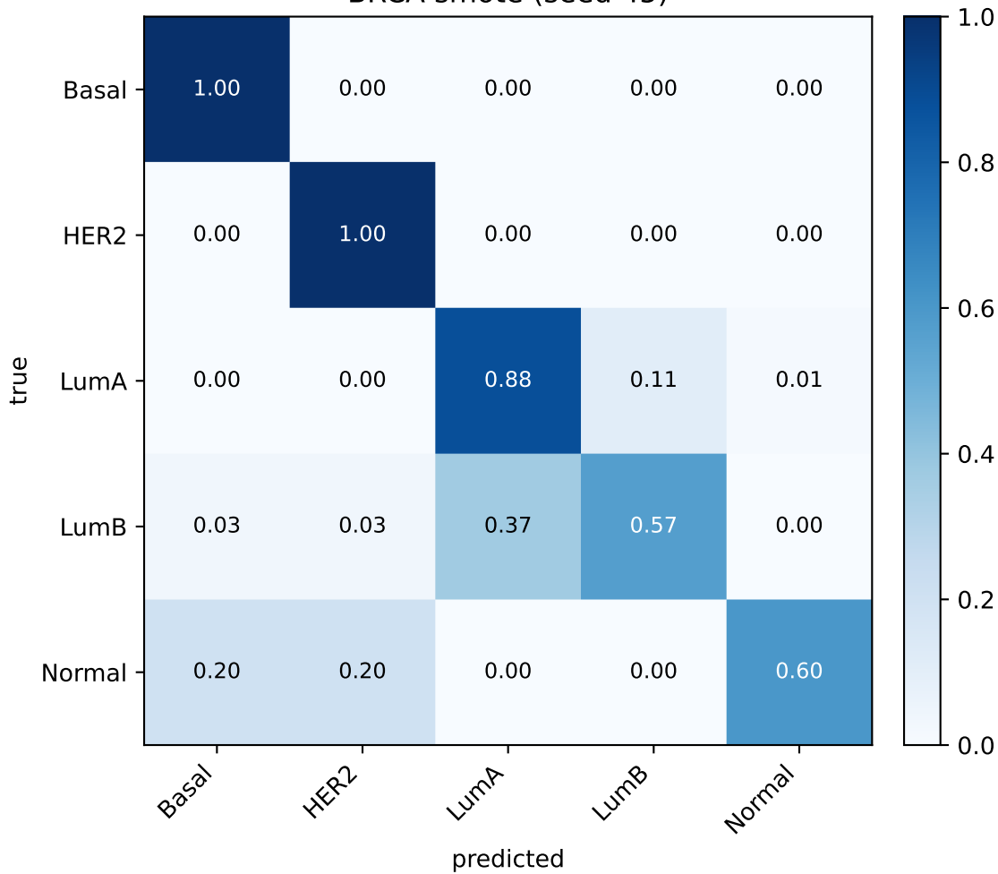
BRCA smote (seed 45)
