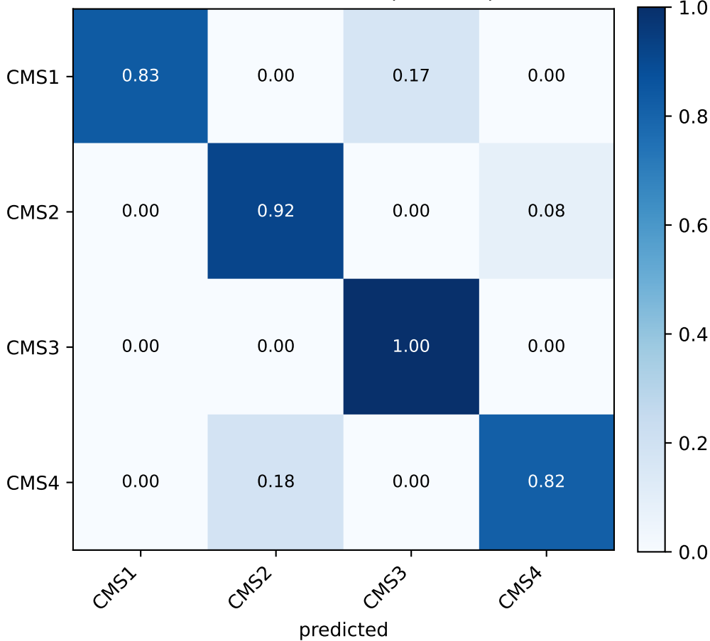
COAD borderline (seed 44)
