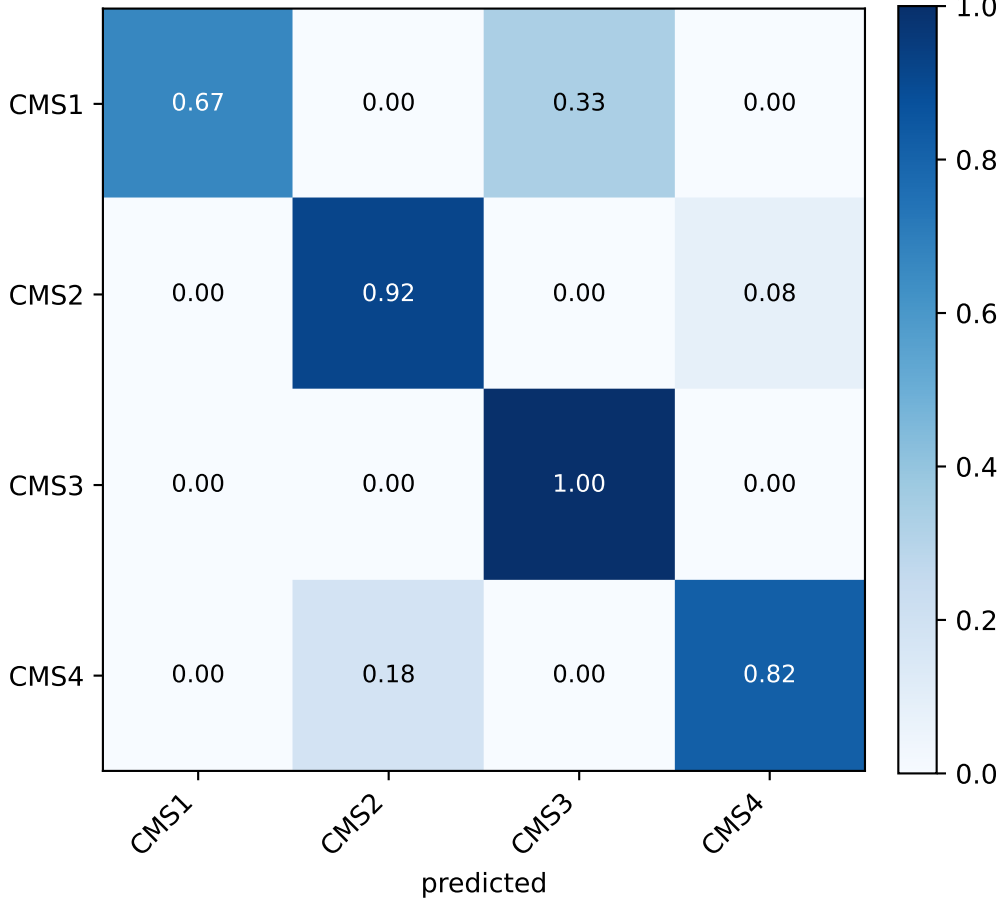
COAD smote (seed 45)
