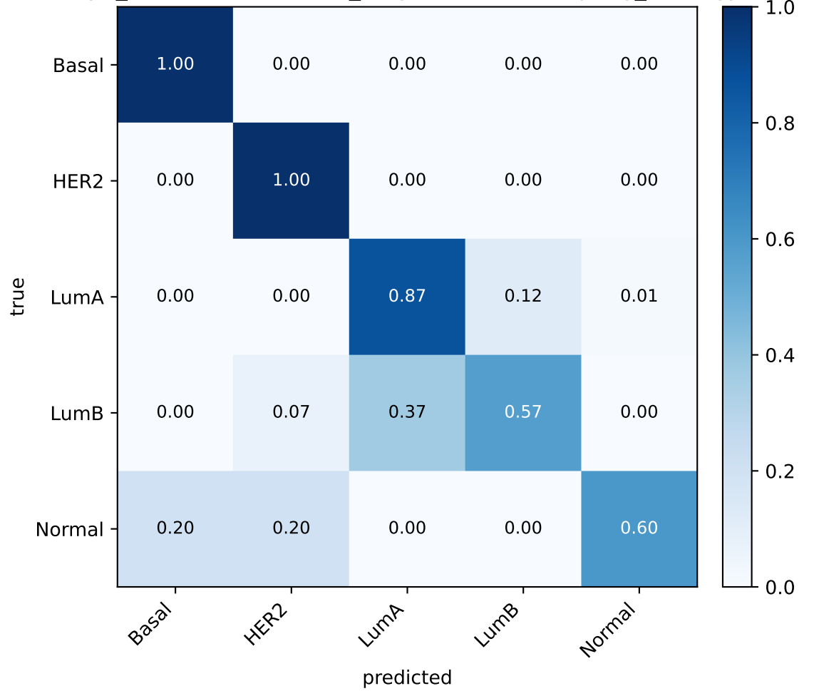
BRCA adasyn_tuned (seed 44, {'k_neighbors': 3, 'sampling_strategy': 'auto'})
