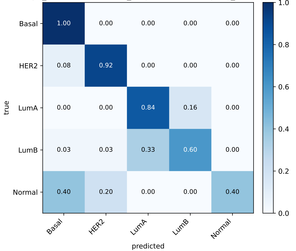
BRCA adasyn_tuned (seed 45, {'k_neighbors': 3, 'sampling_strategy': 'auto'})
