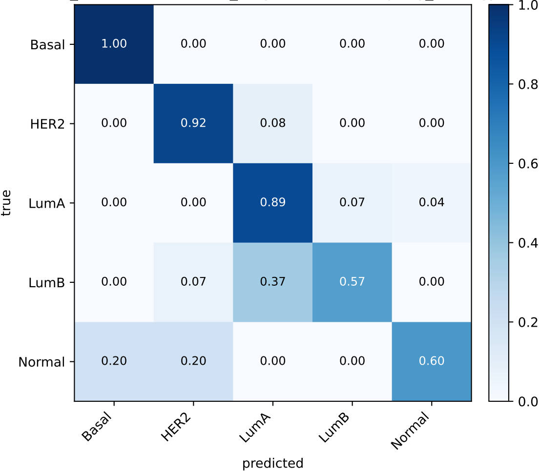
BRCA borderline_tuned (seed 44, {'k_neighbors': 3, 'sampling_strategy': 'minority'})
