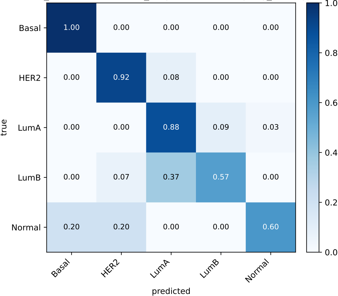
BRCA borderline_tuned (seed 45, {'k_neighbors': 3, 'sampling_strategy': 'minority'})
