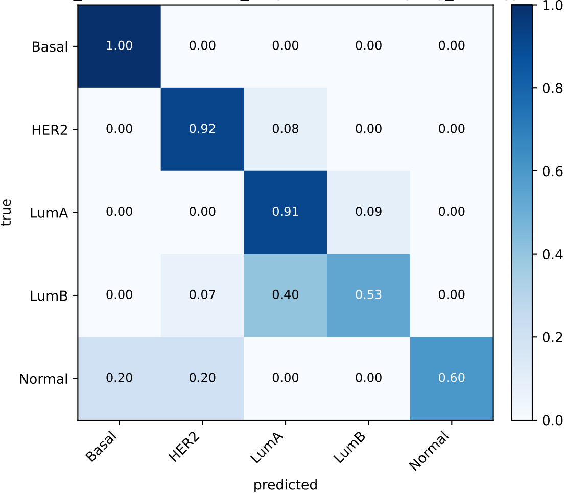
BRCA borderline_tuned (seed 46, {'k_neighbors': 3, 'sampling_strategy': 'minority'})
