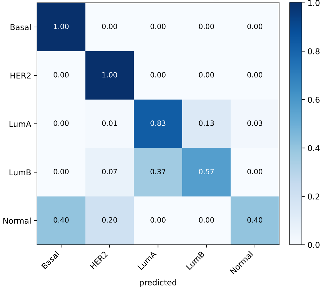
BRCA random_tuned (seed 44, {'sampling_strategy': 'auto'})
