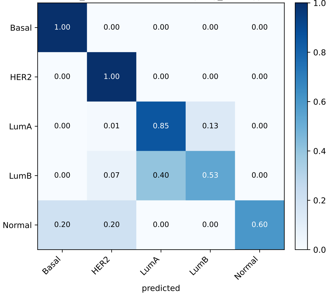
BRCA random_tuned (seed 46, {'sampling_strategy': 'auto'})
