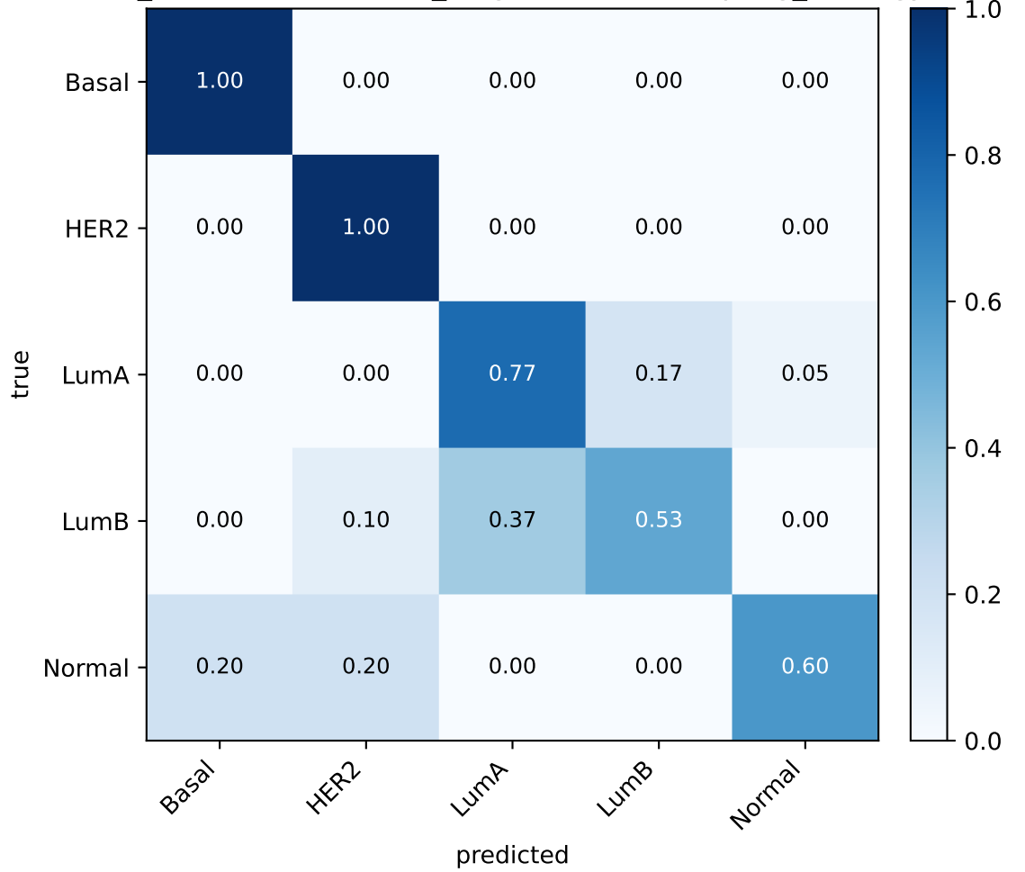
BRCA smote_tuned (seed 42, {'k_neighbors': 3, 'sampling_strategy': 'auto'})
