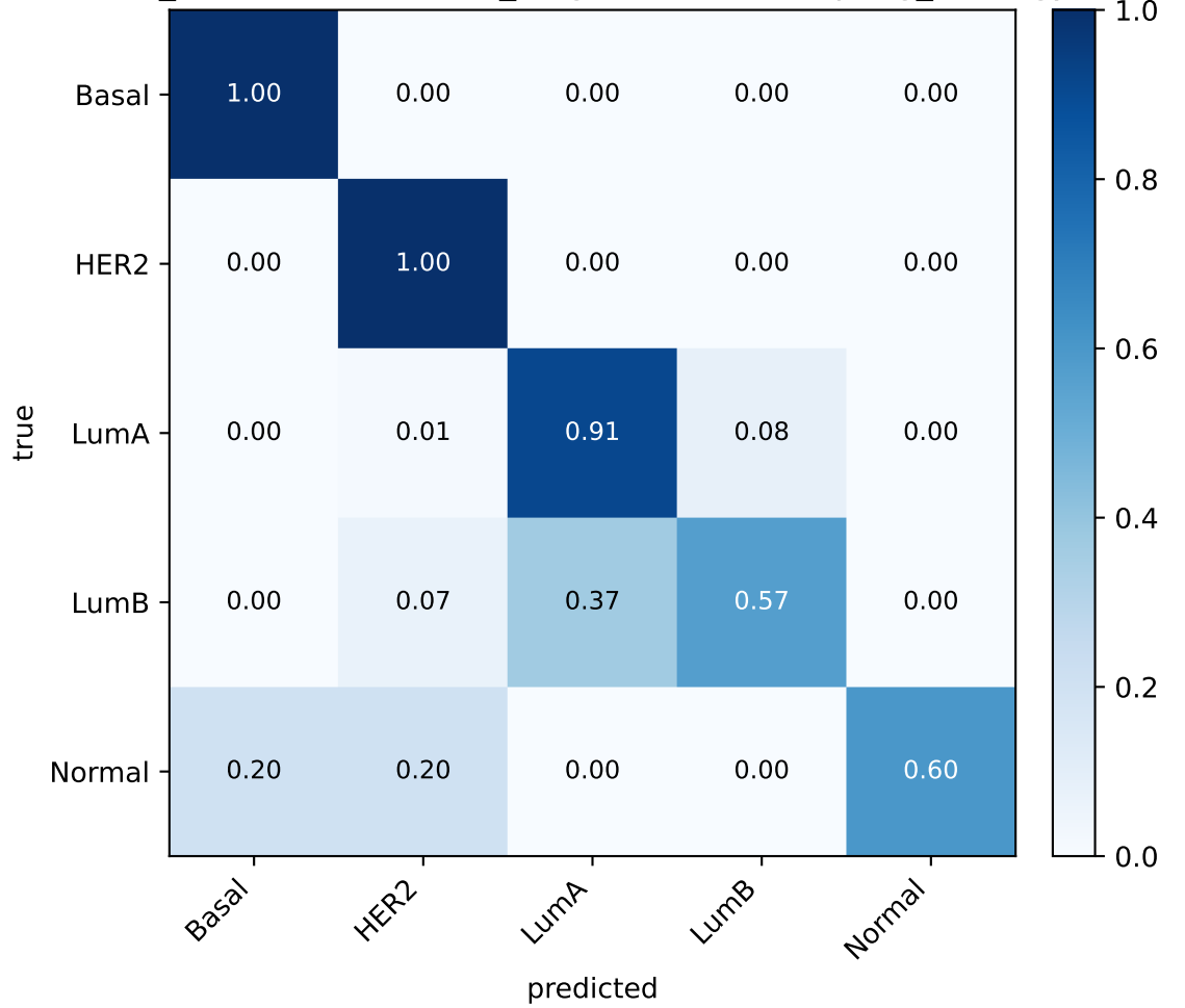
BRCA smote_tuned (seed 43, {'k_neighbors': 3, 'sampling_strategy': 'auto'})
