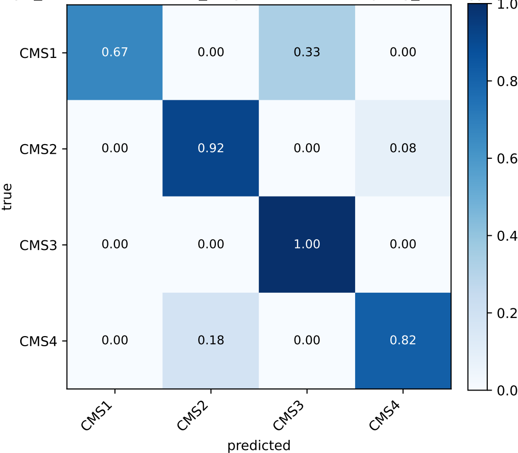
COAD adasyn_tuned (seed 43, {'k_neighbors': 10, 'sampling_strategy': 'minority'})
