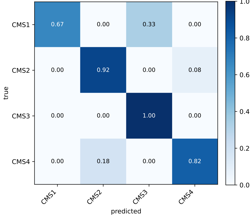
COAD borderline_tuned (seed 44, {'k_neighbors': 5, 'sampling_strategy': 'minority'})
