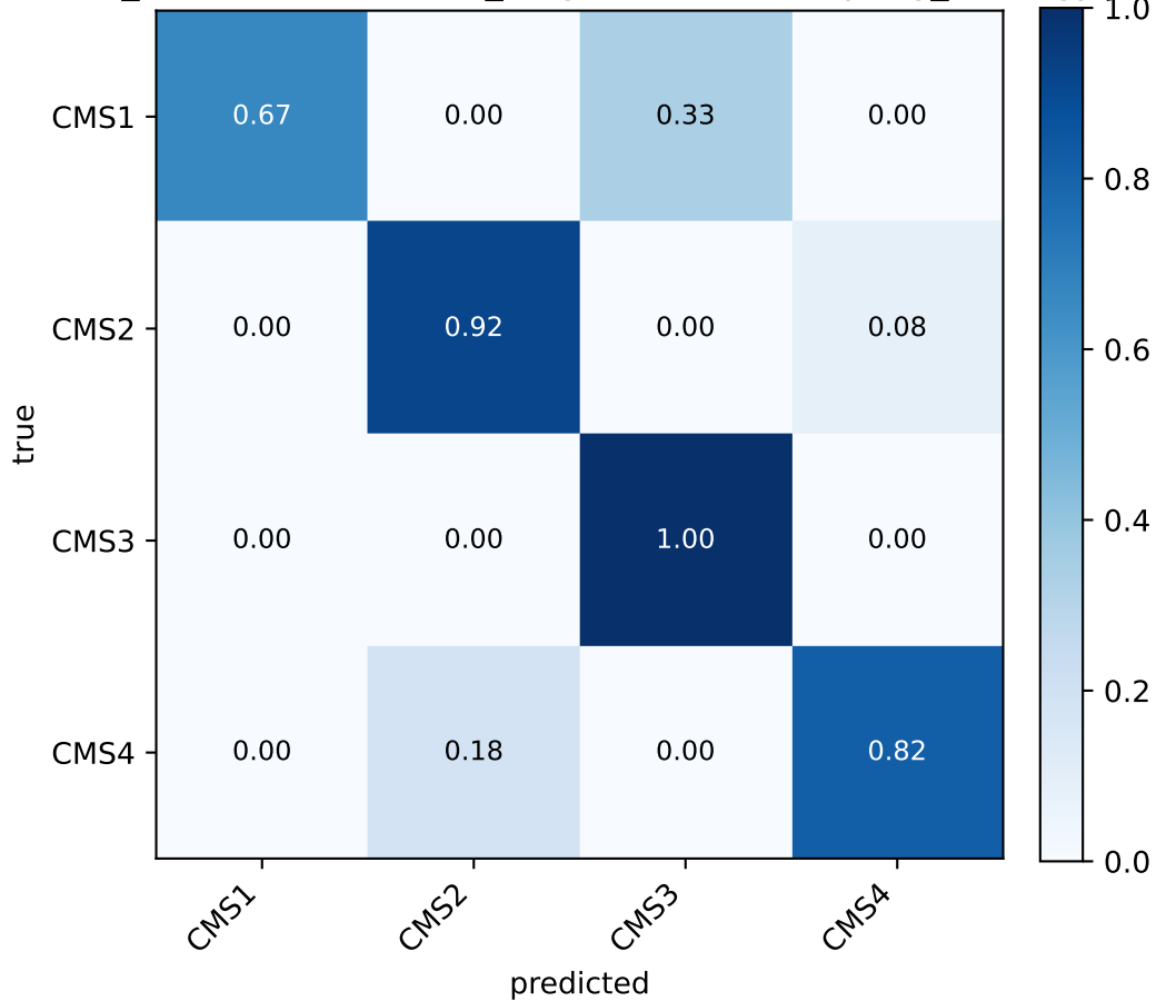
COAD borderline_tuned (seed 46, {'k_neighbors': 5, 'sampling_strategy': 'minority'})
