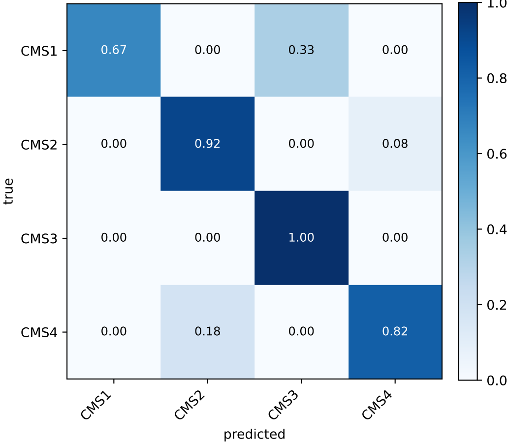
COAD smote_tuned (seed 45, {'k_neighbors': 10, 'sampling_strategy': 'auto'})
