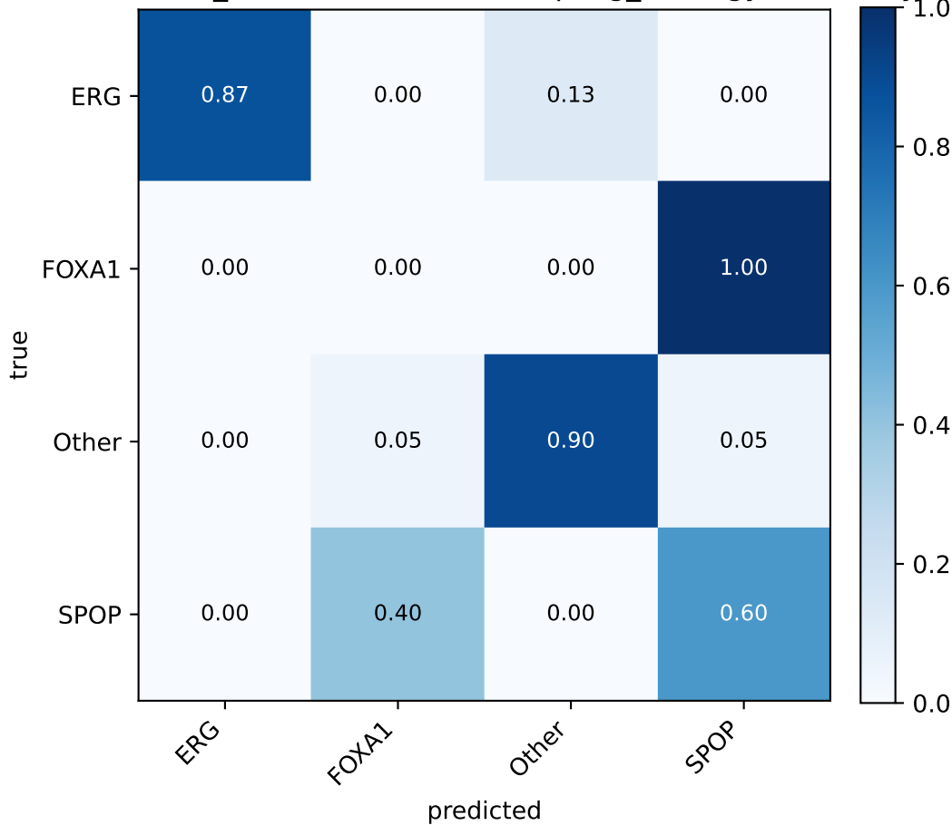
PRAD random_tuned (seed 42, {'sampling_strategy': 'minority'})
