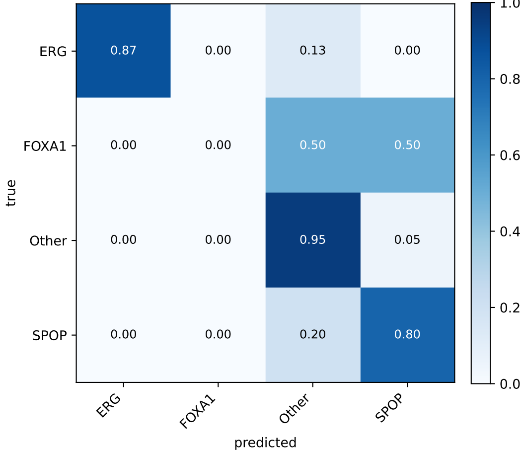
PRAD smote_tuned (seed 42, {'k_neighbors': 5, 'sampling_strategy': 'auto'})
