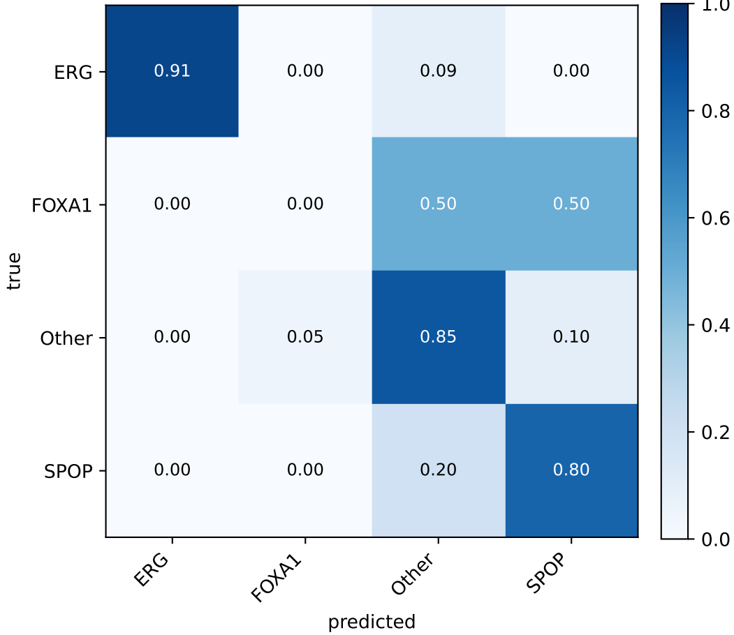
PRAD smote_tuned (seed 45, {'k_neighbors': 5, 'sampling_strategy': 'auto'})
