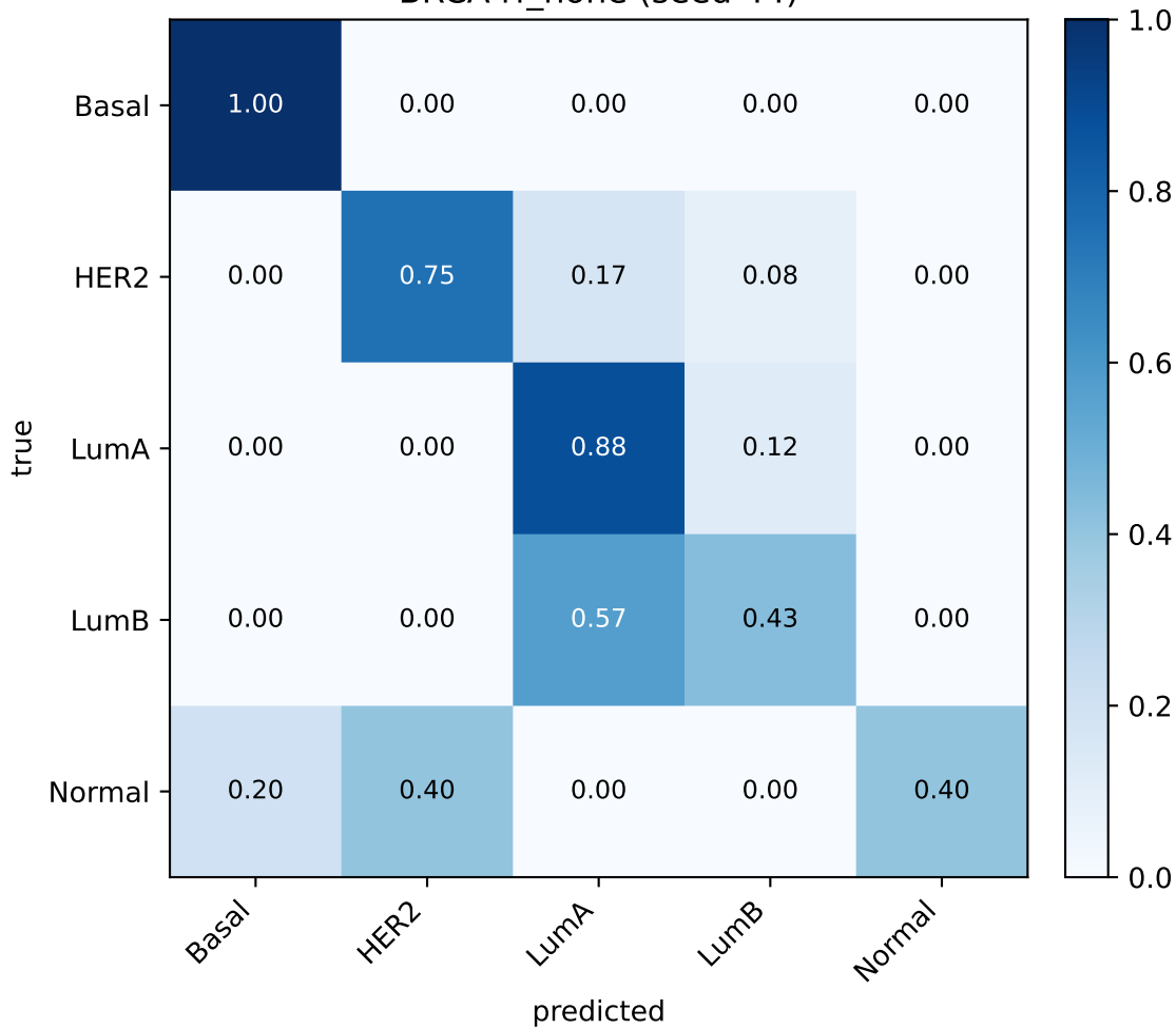
BRCA rf_none (seed 44)
