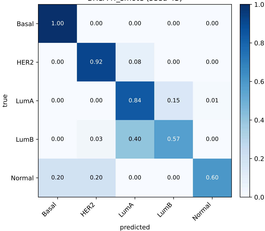
BRCA rf_smote (seed 43)
