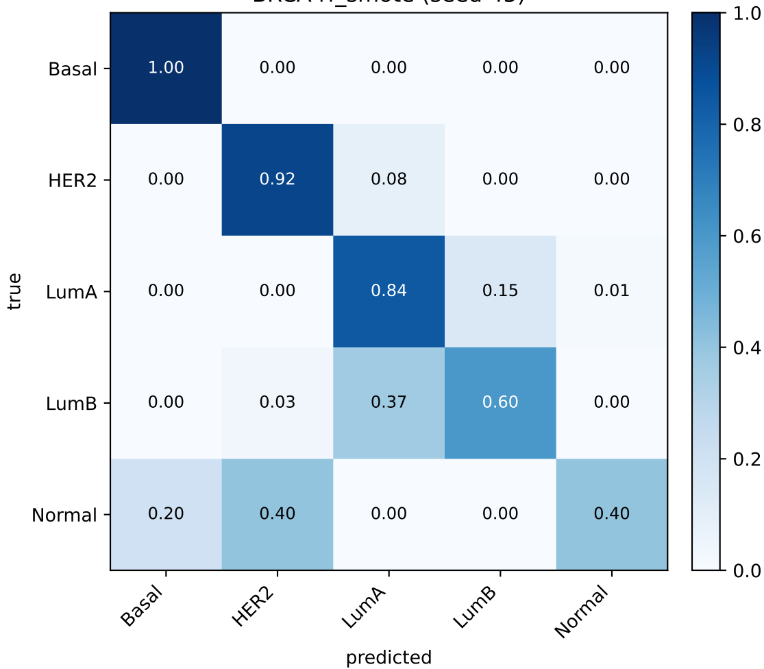
BRCA rf_smote (seed 45)
