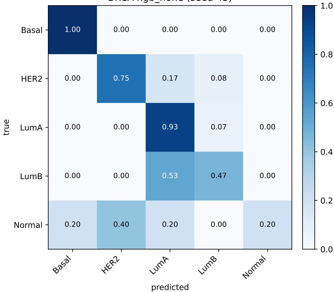
BRCA xgb_none (seed 43)
