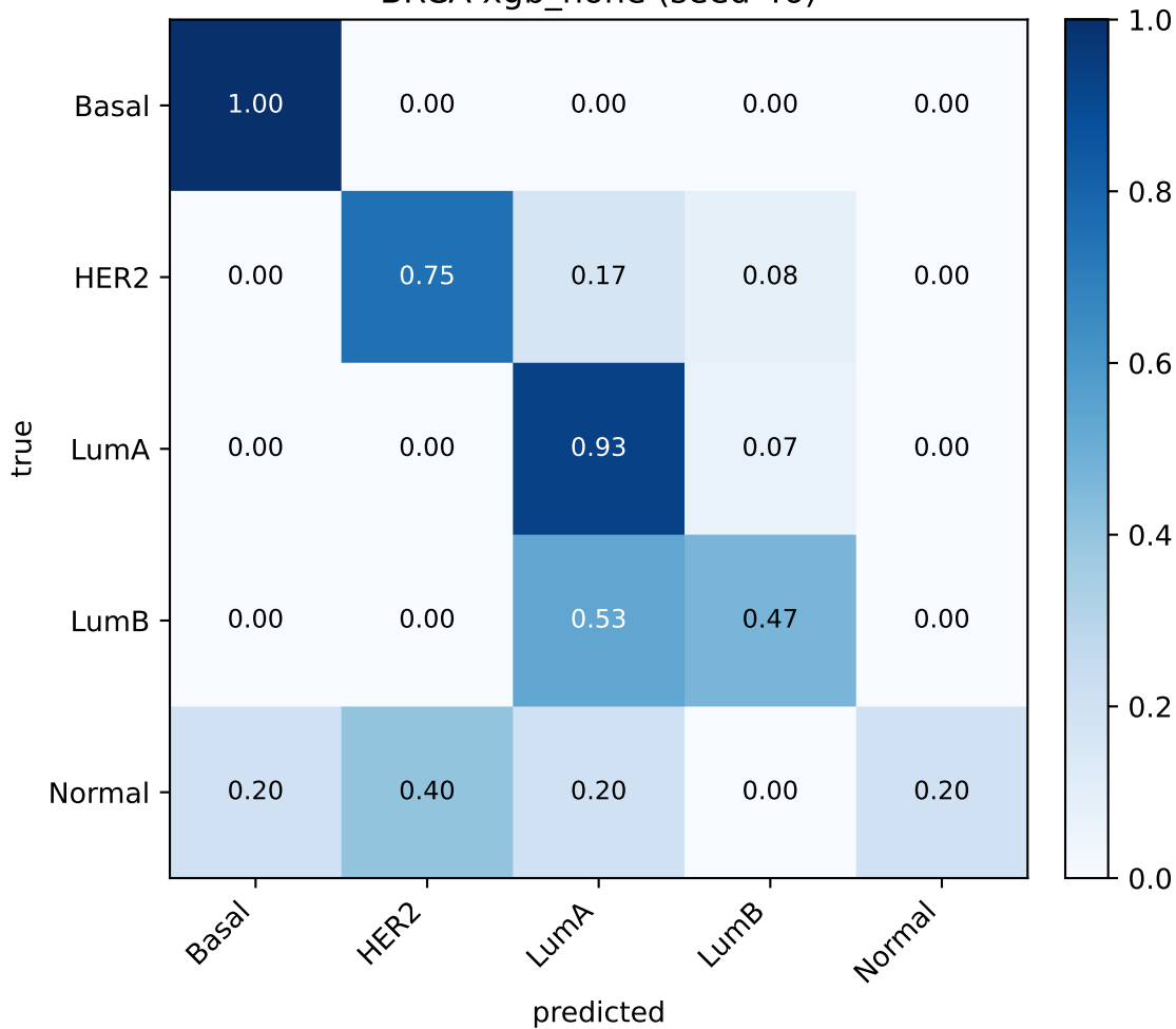
BRCA xgb_none (seed 46)
