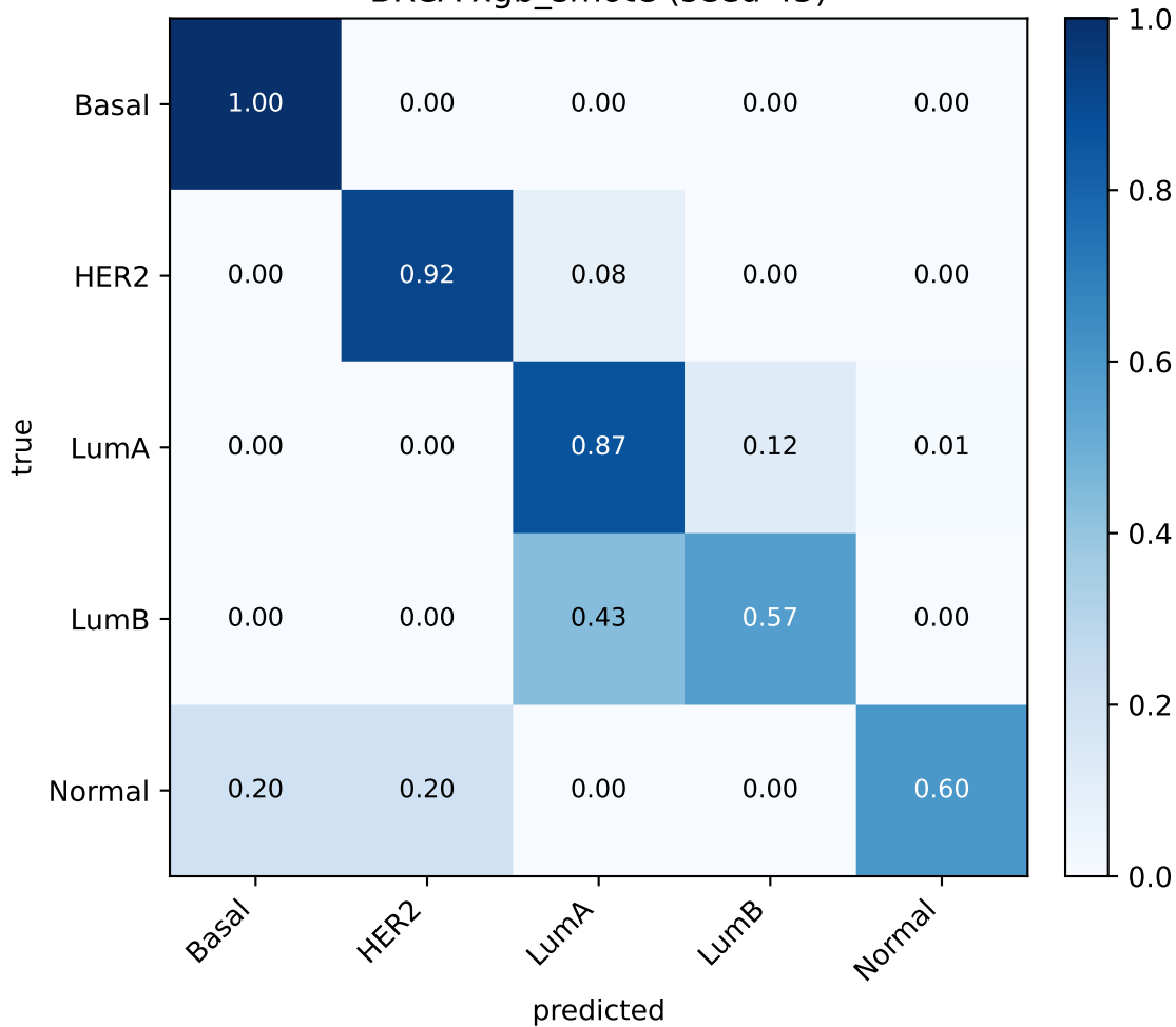
BRCA xgb_smote (seed 45)
