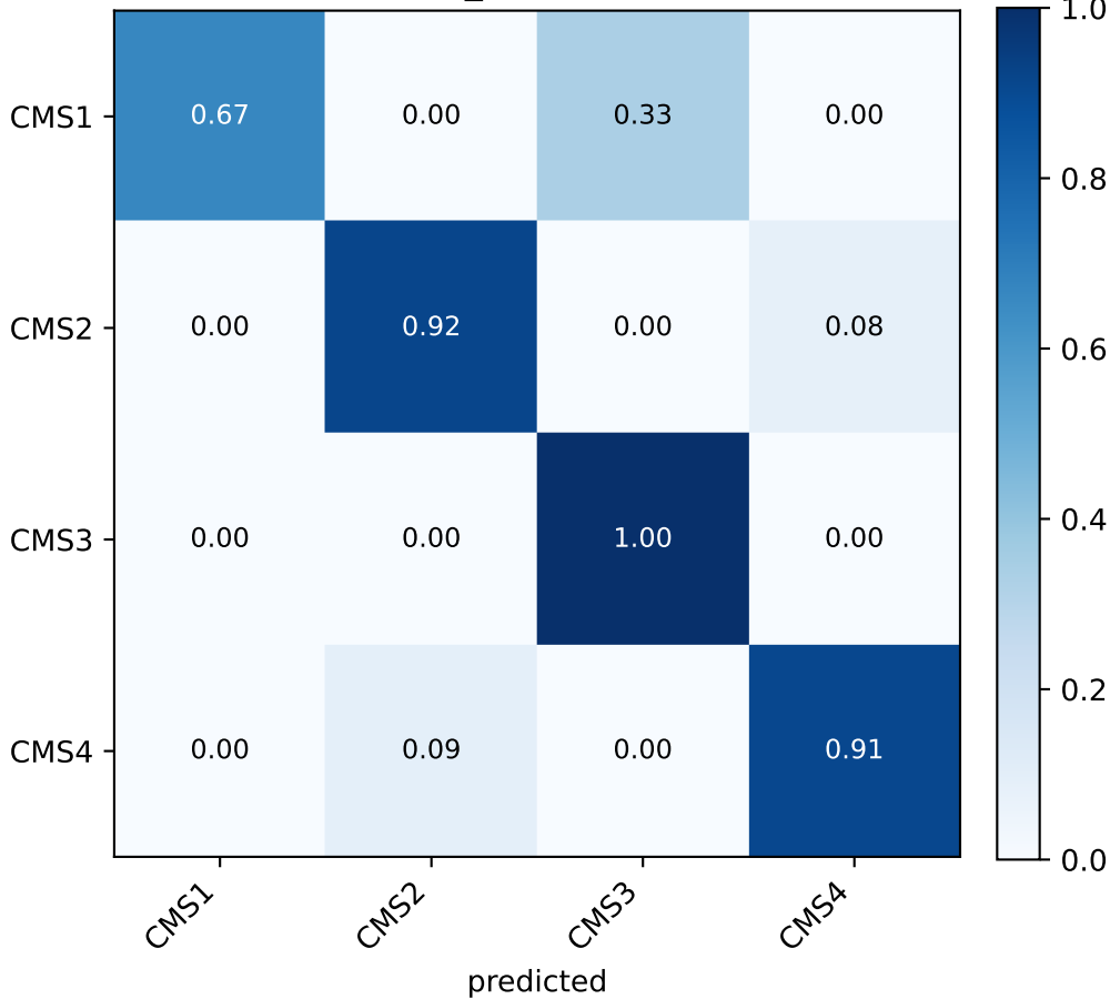
COAD rf_none (seed 43)
