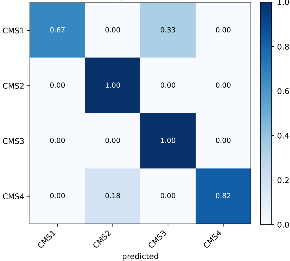
COAD rf_smote (seed 44)
