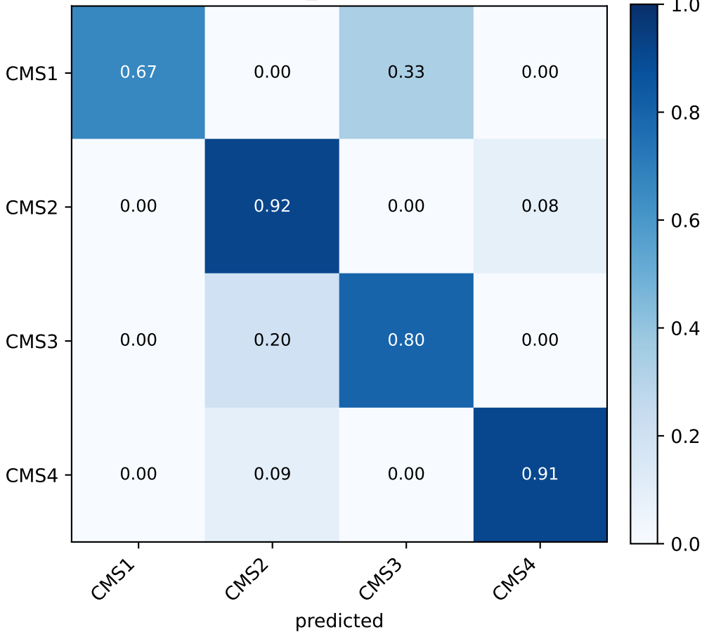
COAD xgb_none (seed 42)
