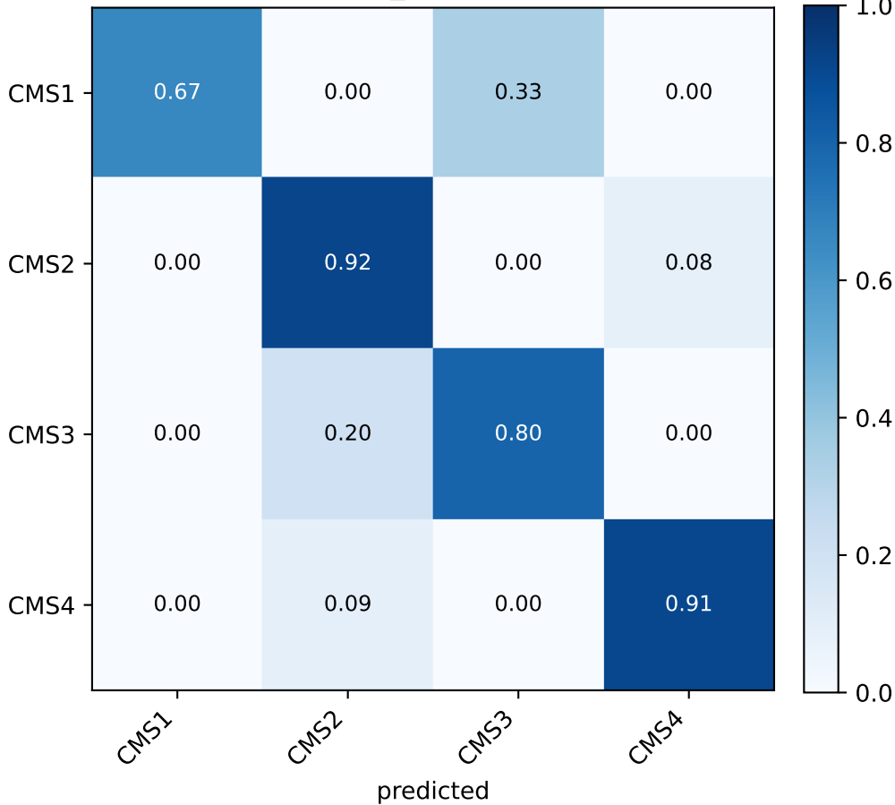
COAD xgb_none (seed 46)
