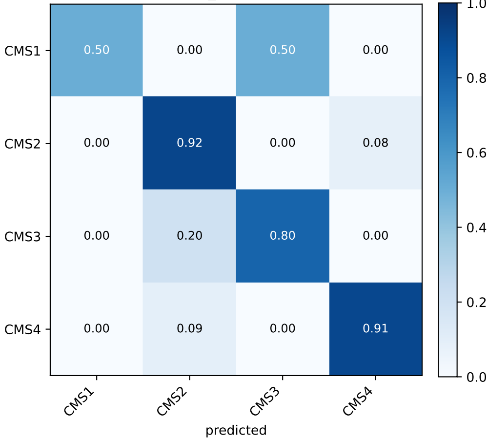
COAD xgb_smote (seed 42)
