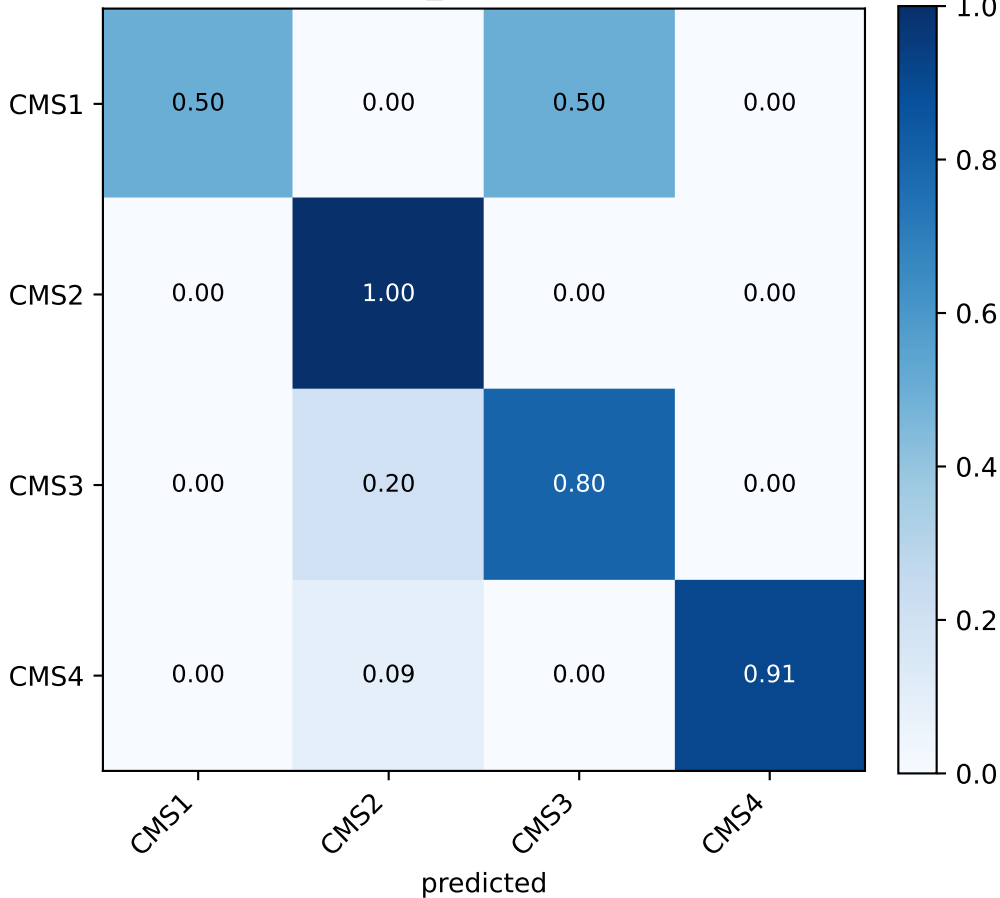
COAD xgb_smote (seed 46)
