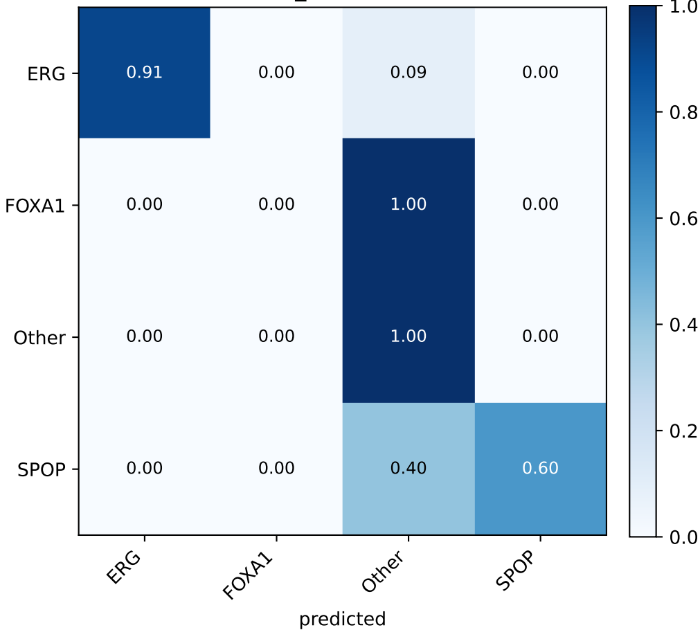
PRAD rf_none (seed 42)
