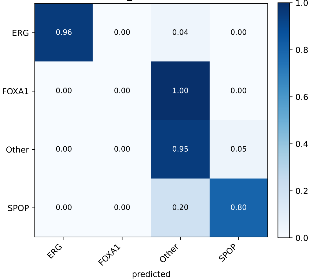
PRAD rf_smote (seed 43)
