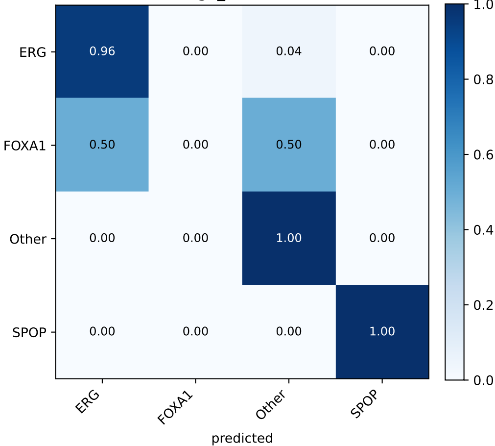
PRAD xgb_none (seed 43)
