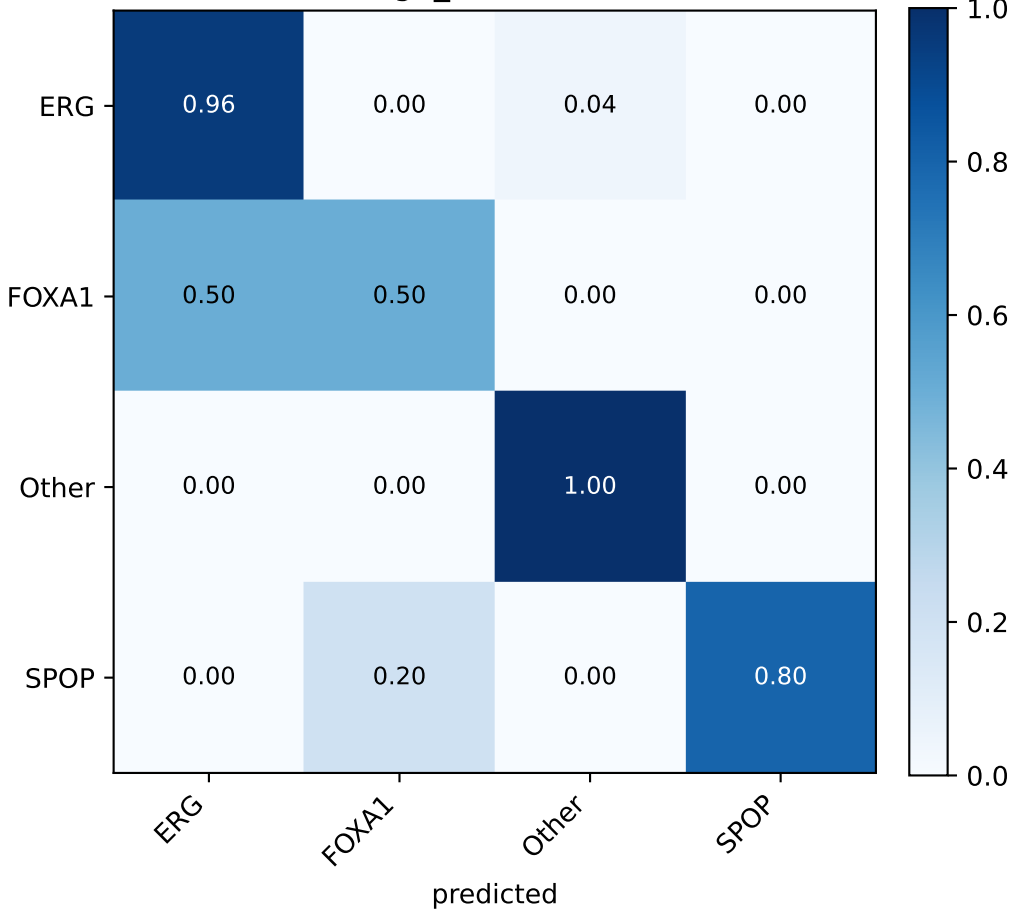
PRAD xgb_smote (seed 45)
