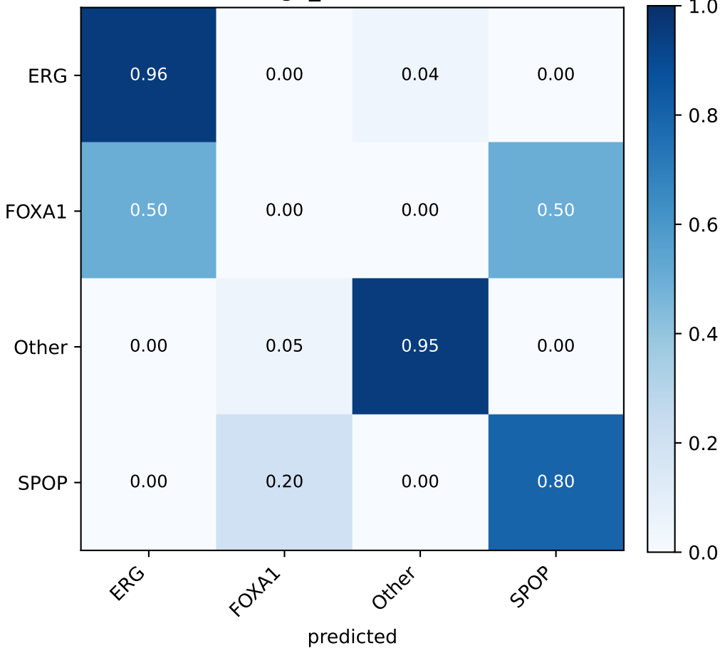
PRAD xgb_smote (seed 46)
