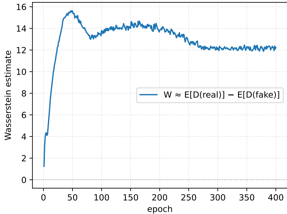
BRCA WGAN-GP — Wasserstein estimate
