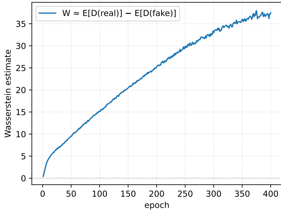
COAD WGAN-GP — Wasserstein estimate
