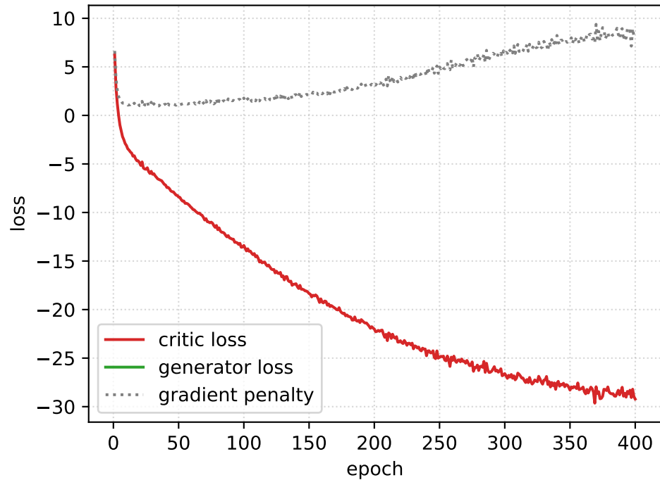
COAD WGAN-GP — D / G / GP
