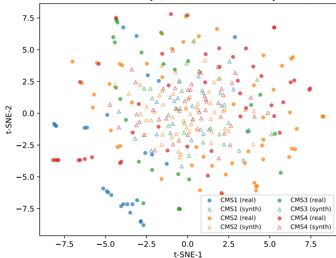
COAD t-SNE overlay (real train vs WGAN-GP synthetic)
