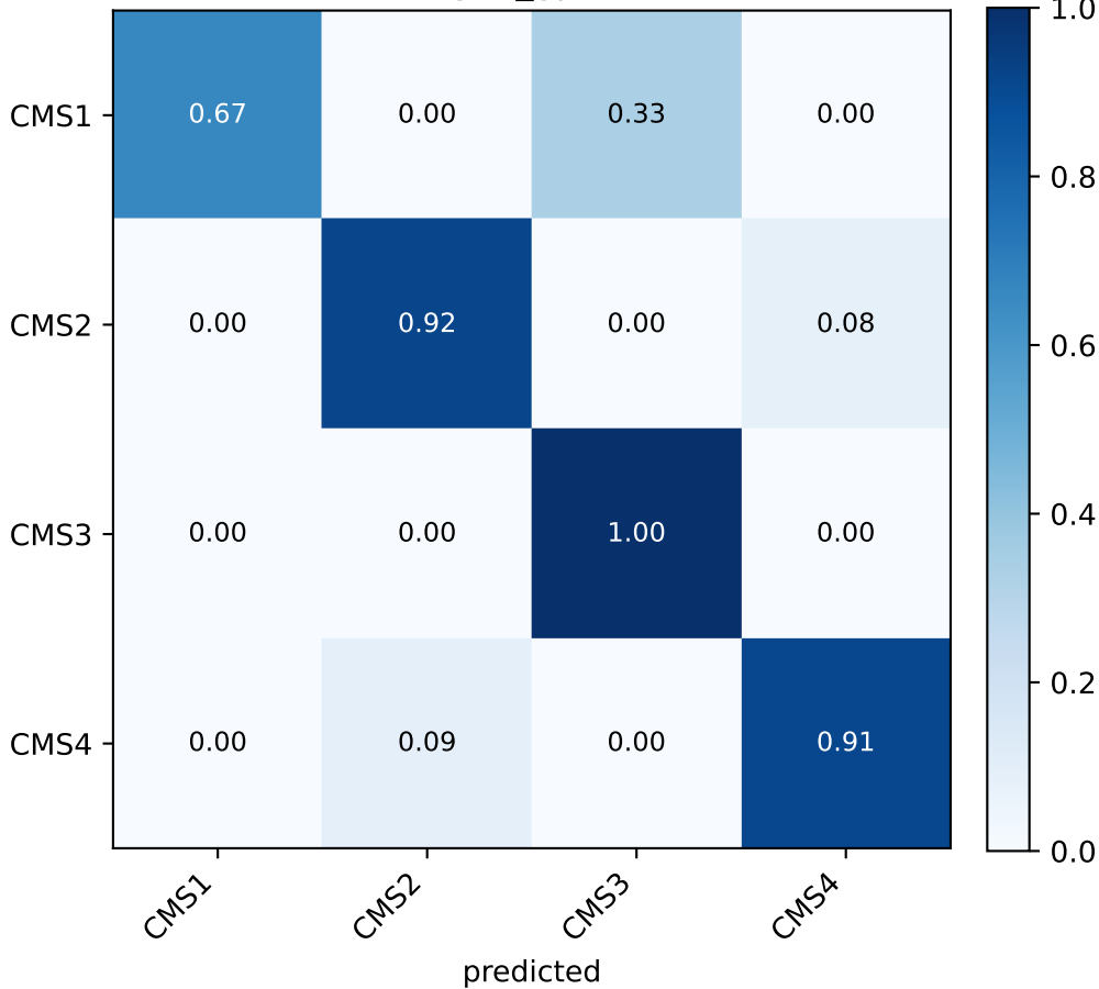
COAD wgan_gp (seed 45)
