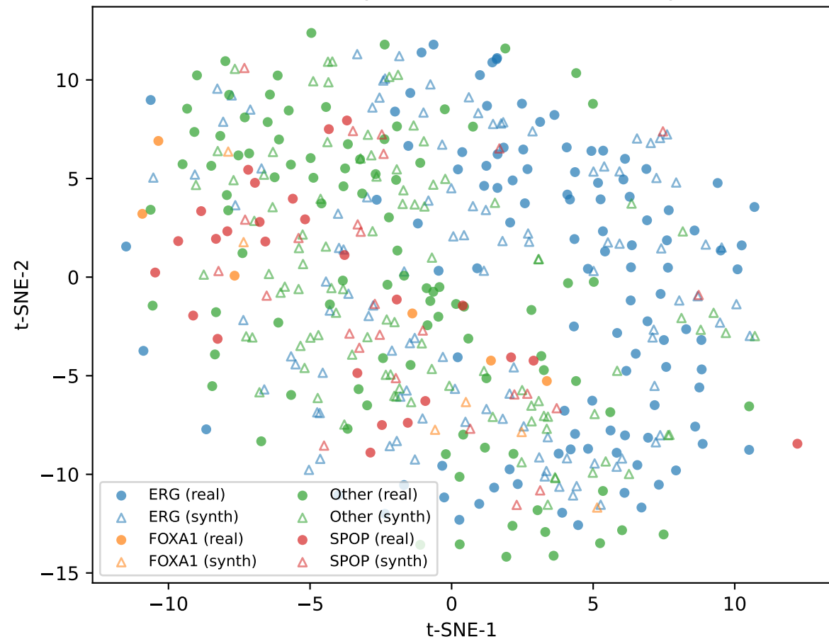
PRAD t-SNE overlay (real train vs WGAN-GP synthetic)
