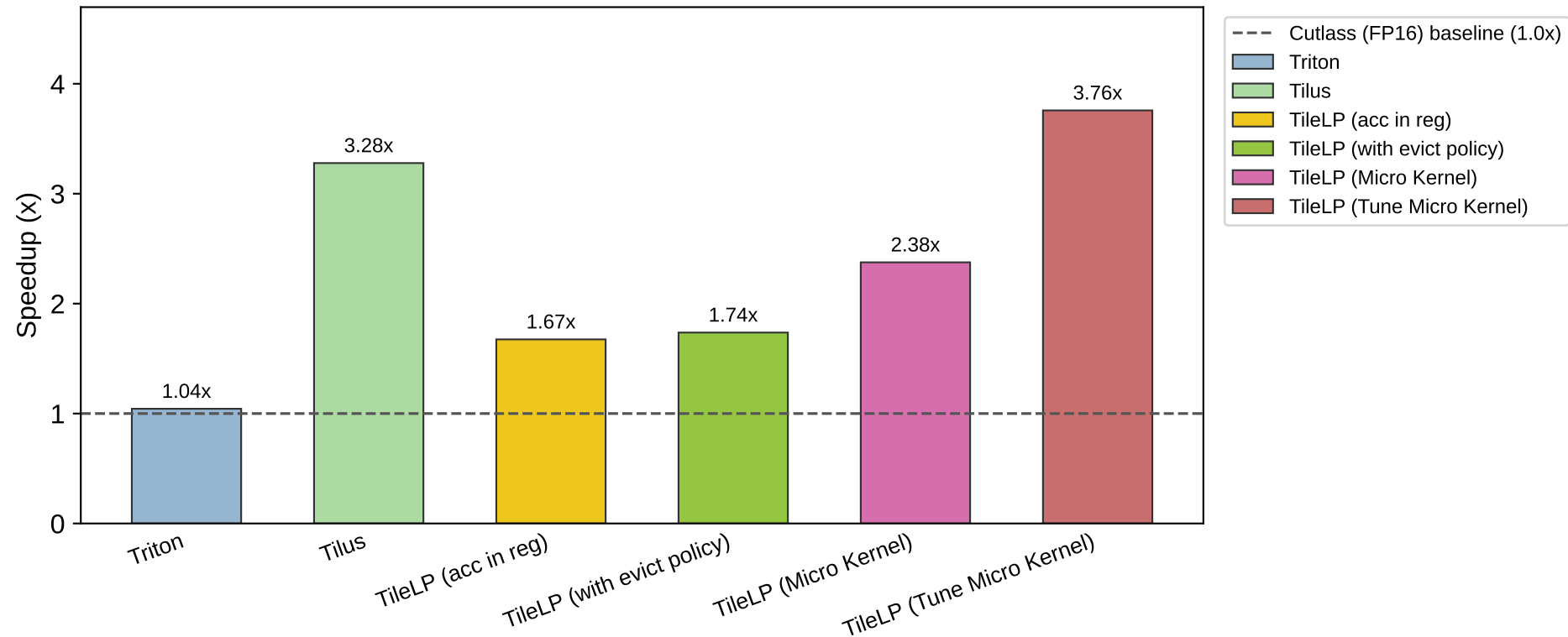
Ablation Breakdown (m=1, k=8192, n=57344, W4A16, group=128)
