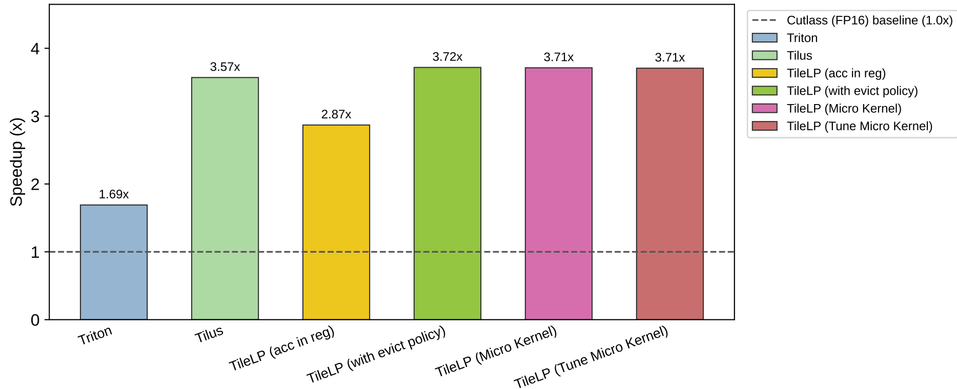
Ablation Breakdown (m=1, k=28672, n=8192, W4A16, group=128)
