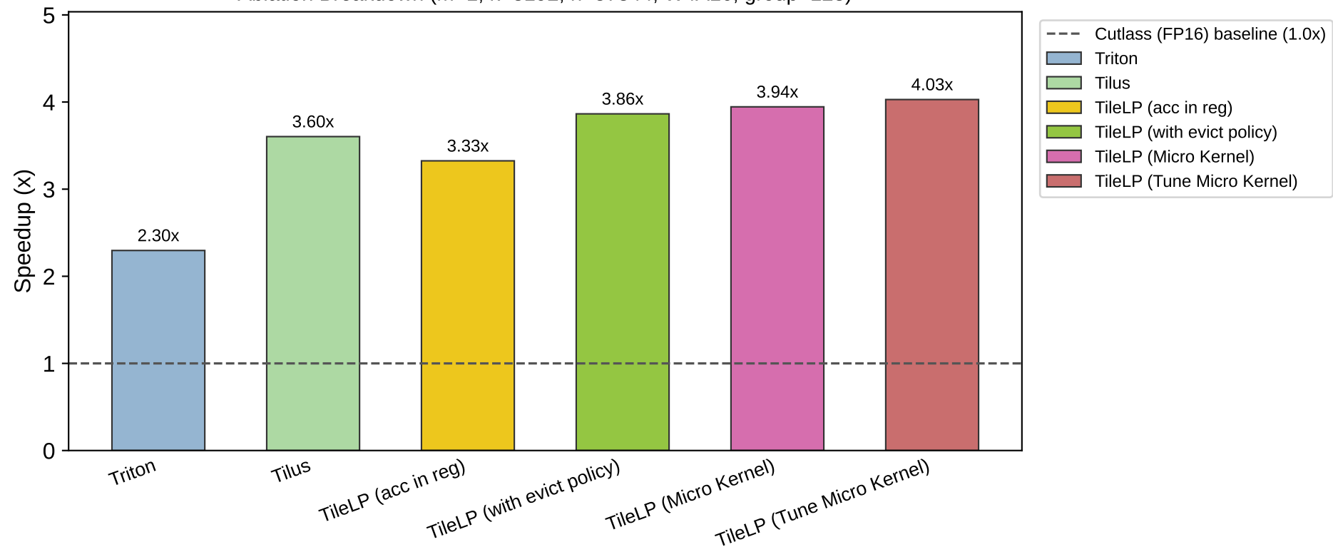
Ablation Breakdown (m=1, k=8192, n=57344, W4A16, group=128)
