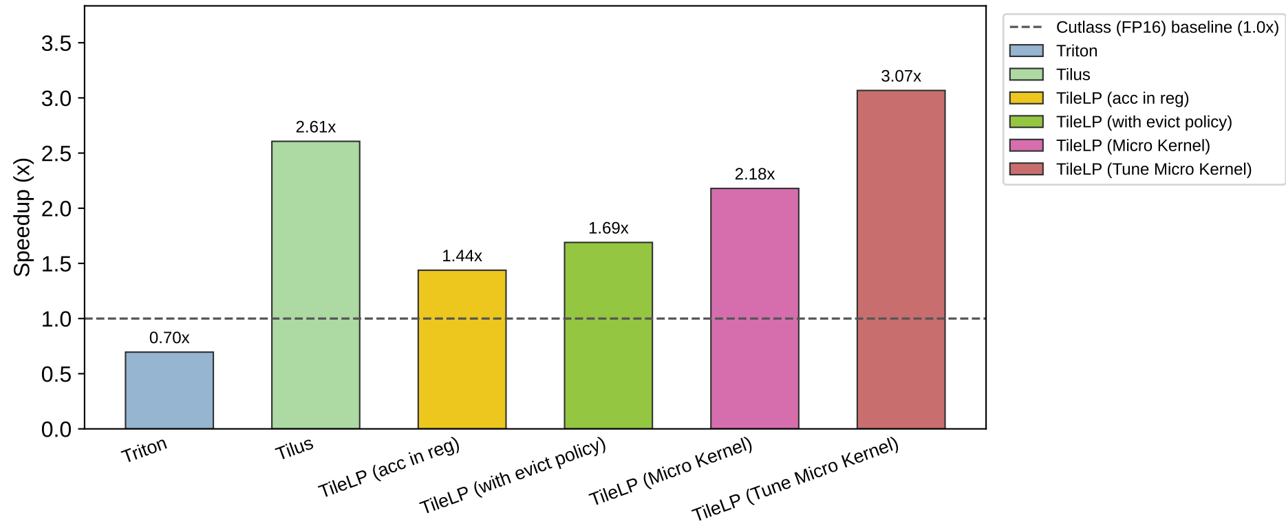
Ablation Breakdown (m=1, k=8192, n=8192, W4A16, group=128)
