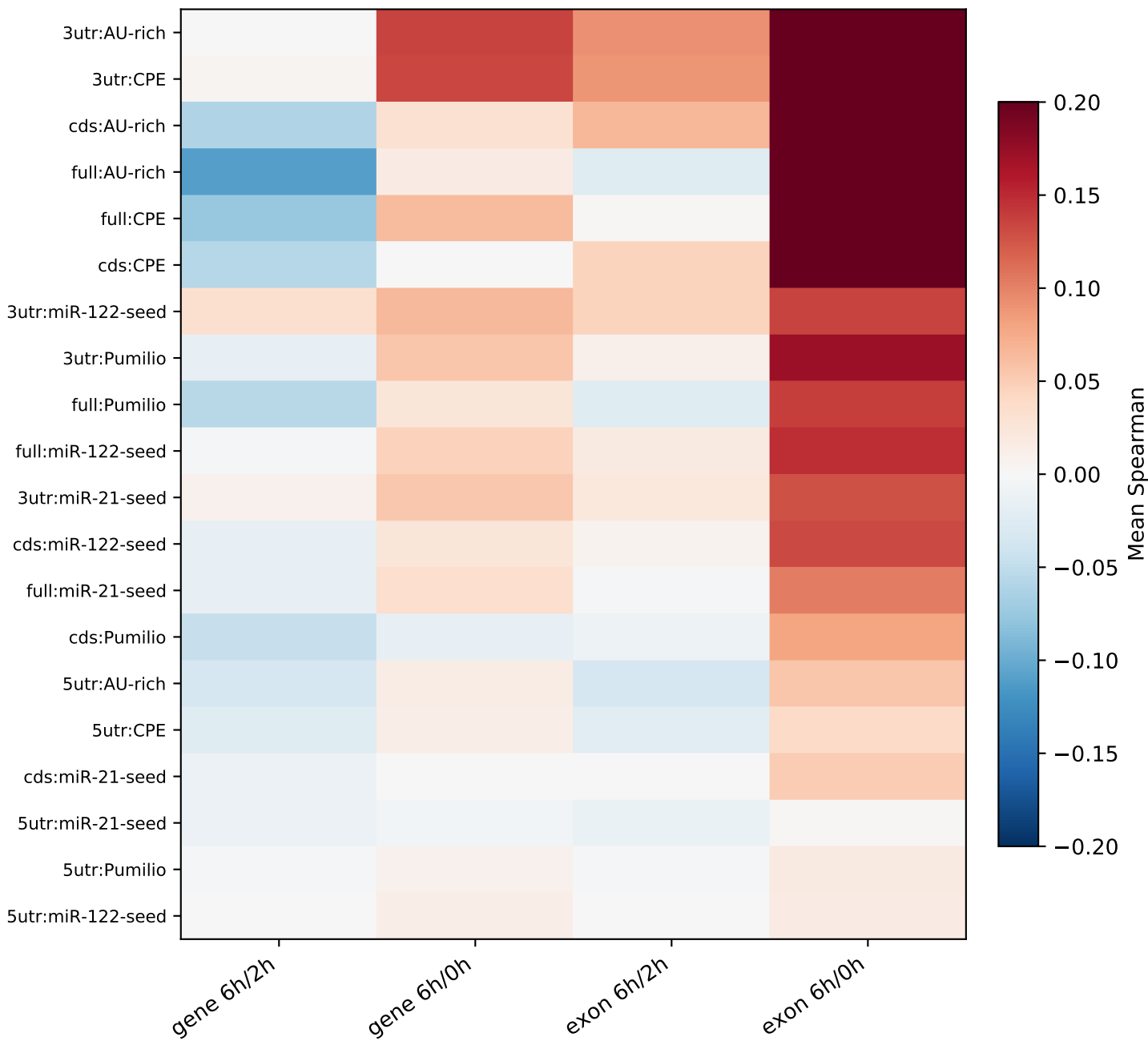
Seed motif and AU-rich feature associations
