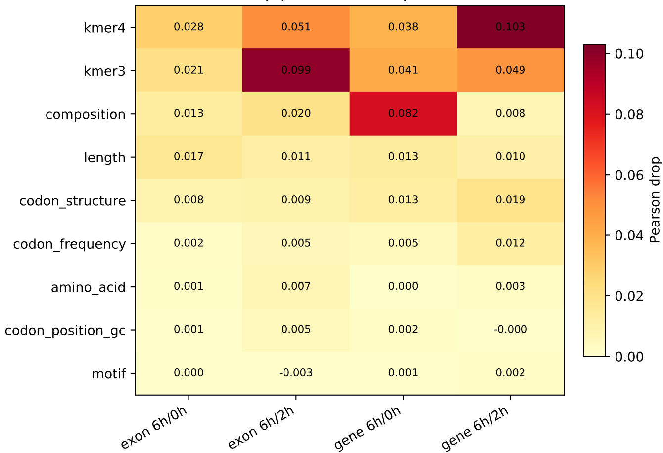
Group permutation importance
