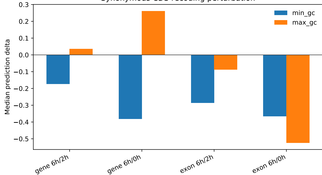
Synonymous CDS recoding perturbation
